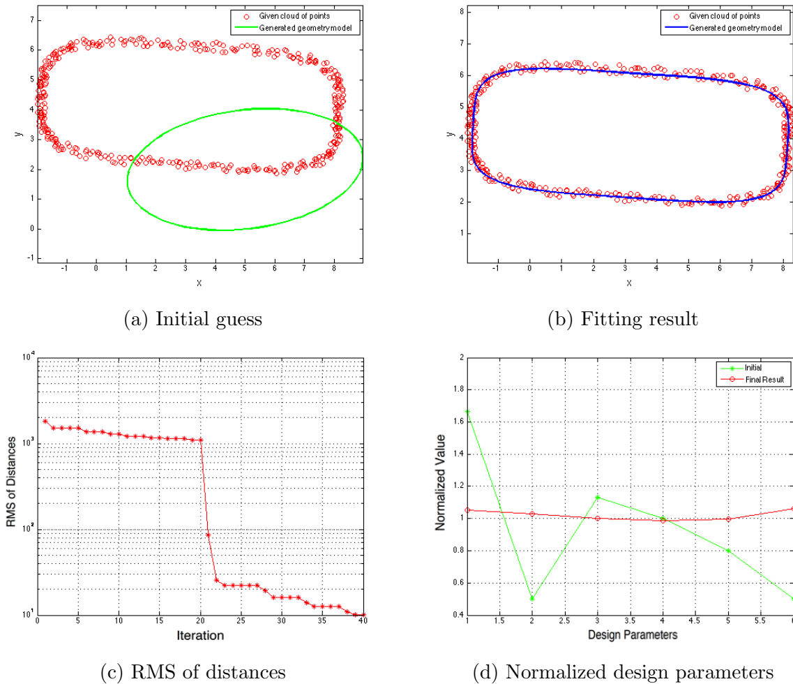
Figure 4.29: Super-ellipse fitting result based on the noisy points data 2
