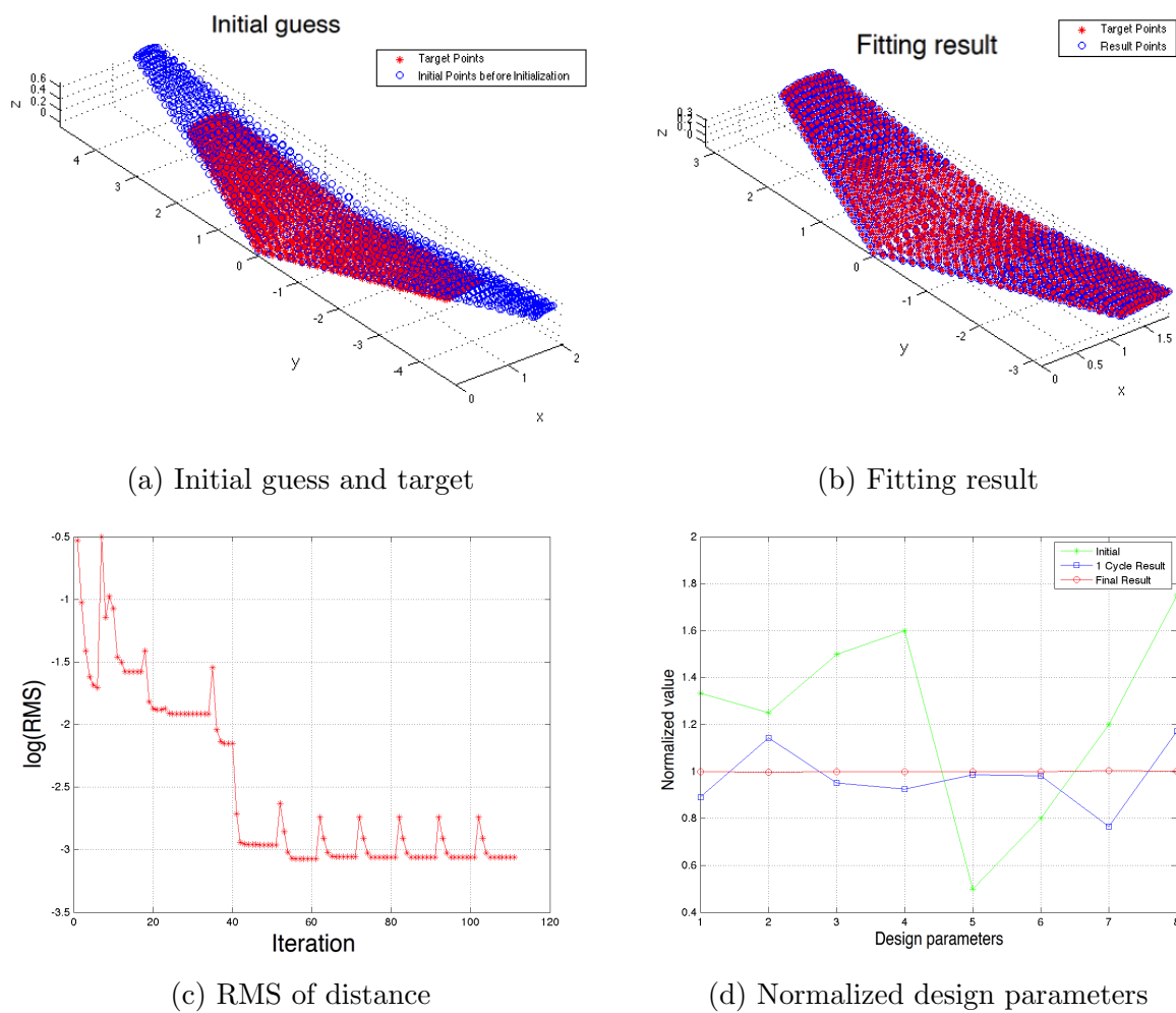
Figure 5.4: Wing fitting results
