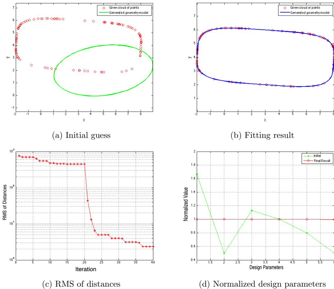
Figure 4.27: Super-ellipse fitting result based on the non-uniform space points data 3
