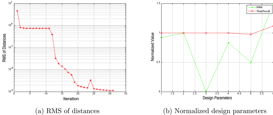
Figure 4.11: Airfoil fitting results analysis
