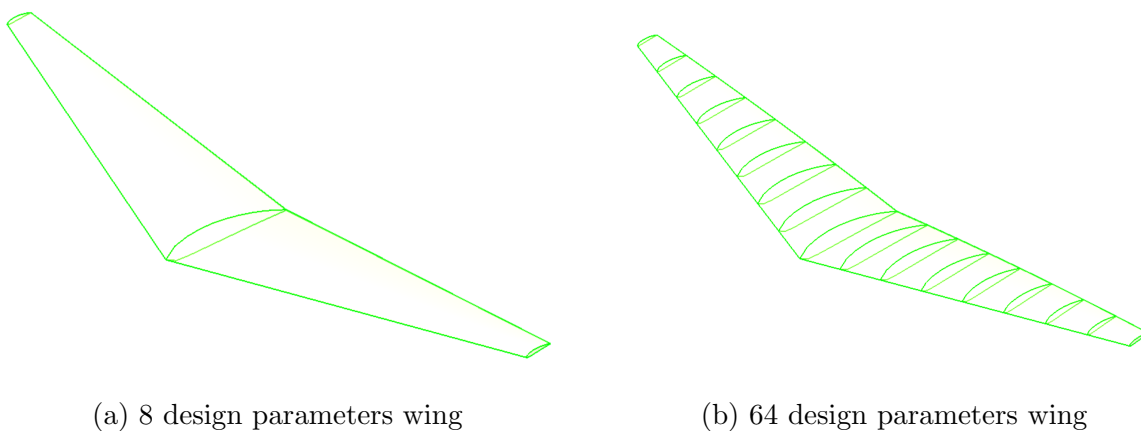
Figure 5.16: Different number of design parameters for the wing generation
