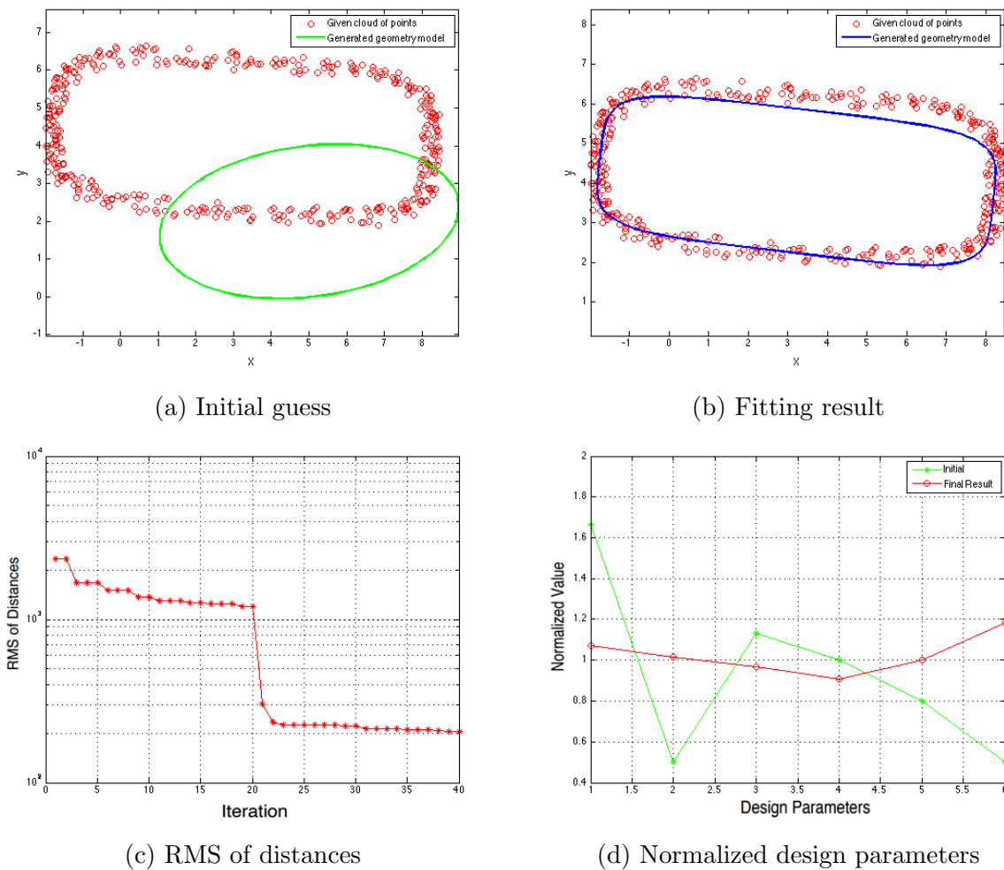
Figure 4.30: Super-ellipse fitting result based on the noisy points data 3
