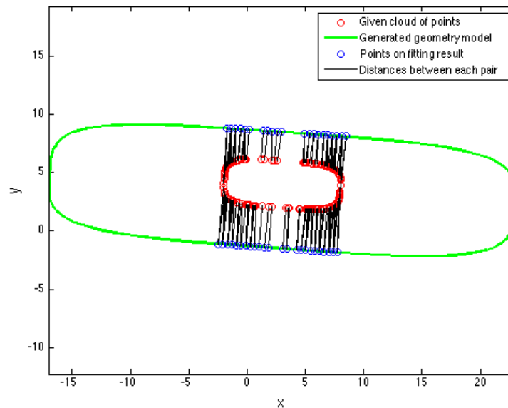
Figure 4.12: Initialization based on too large initial guess
