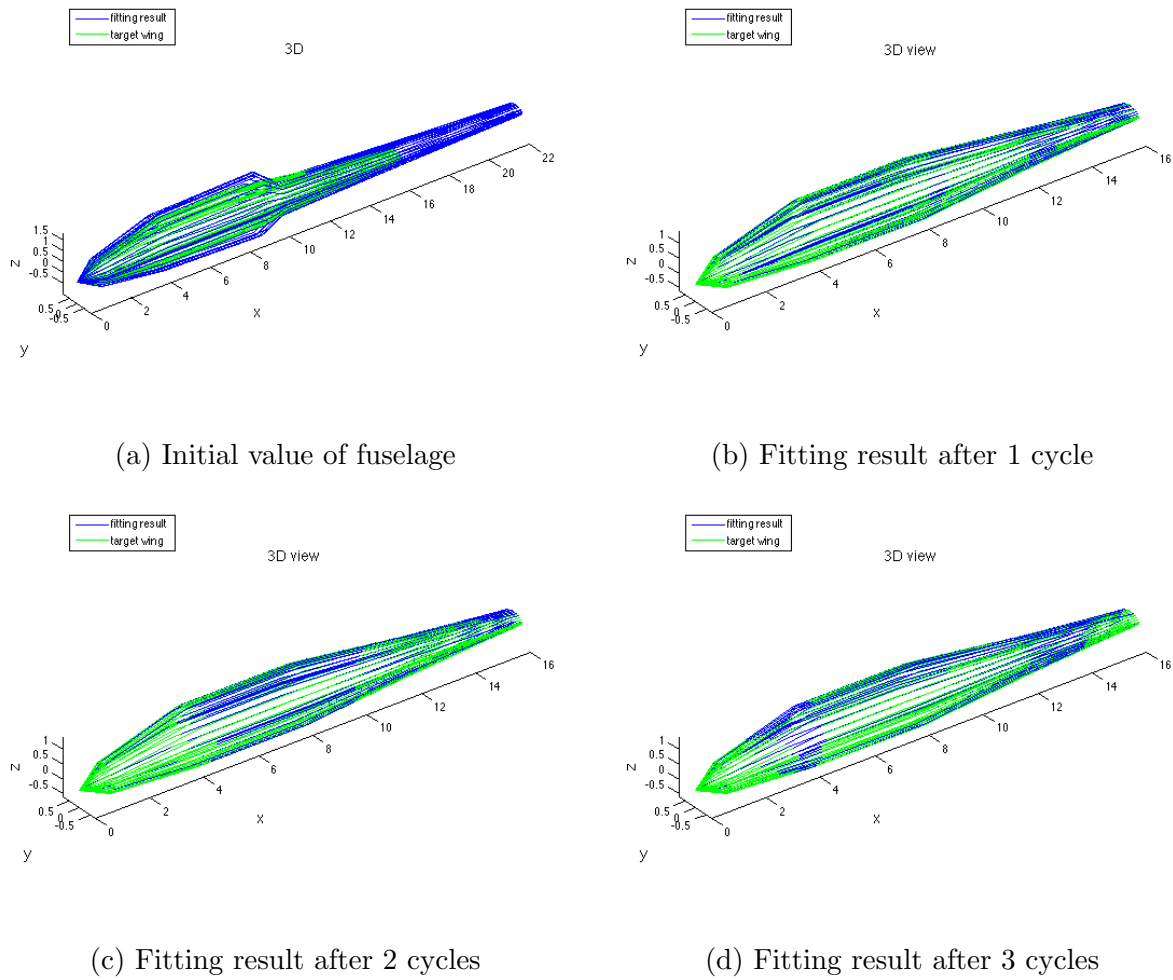
Figure 4.34: Progression of fitting results for 3D fuselage
