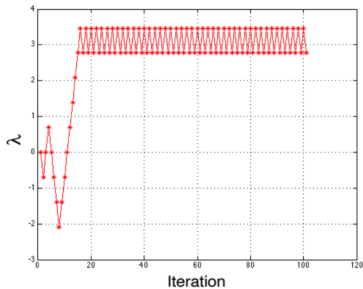
Figure 2.17: \lambda values at each iteration based on ILM
