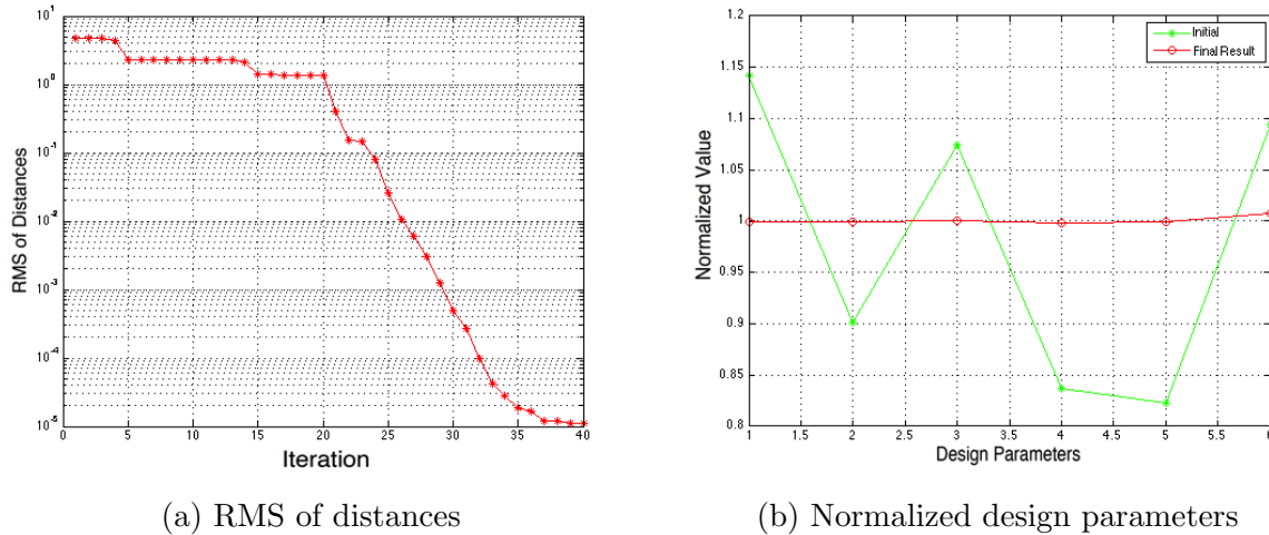
Figure 4.9: Fitting results analysis after using reinitialization technique
