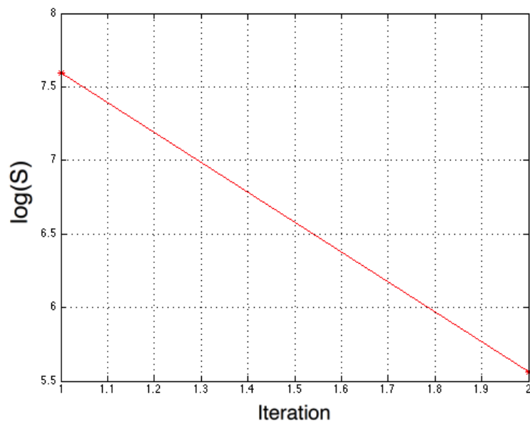
Figure 2.11: Log of objective function value at each iteration based on Newton's method
